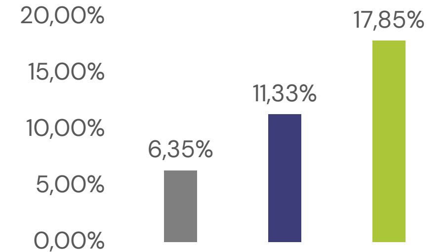
Sharpe Ratio
