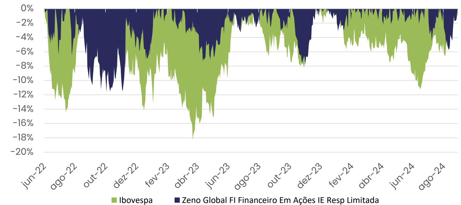
Drawdown (%)
